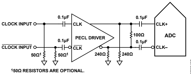
Figure 54. Differential PECL Sample Clock
