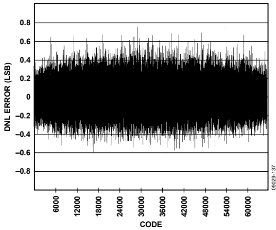
Figure 35. DNL, f_{IN} = 4.3 MHz, 2.5 V p-p FS, AD9467-200
