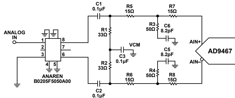
Figure 51. Wideband Balun-Coupled Configuration for IF Applications Up Greater Than 100 MHz
