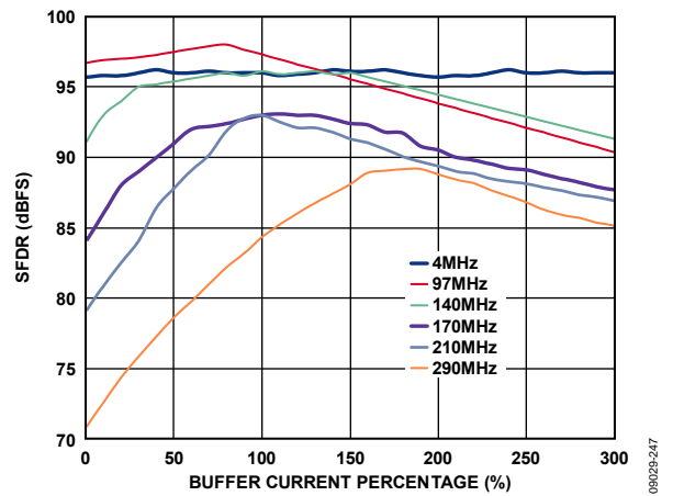
Figure 45. SFDR Performance vs. Buffer Current Percentage Over Analog Input Frequency, AD9467-200
