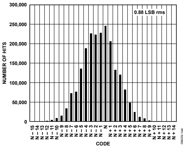
Figure 42. Input-Referred Noise Histogram, 2.5 V p-p FS, AD9467-250
