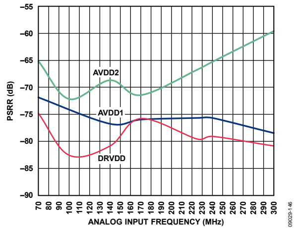
Figure 44. Power Supply Rejection (PSR), AD9467-250
