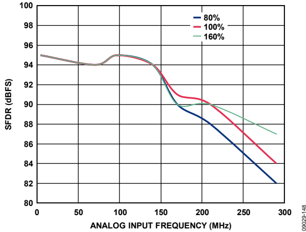
Figure 48. Buffer Current Sweeps, 2.5 V p-p, AD9467-200
