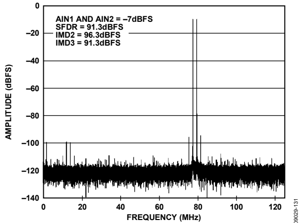
Figure 29. Two-Tone FFT with f_{IN1} = 170 MHz and f_{IN2} = 172 MHz, 2.5 V p-p FS, AD9467-250
