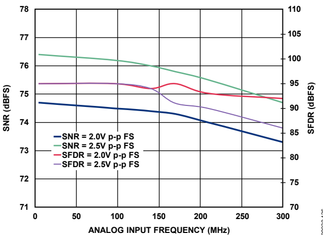
Figure 24. SNR/SFDR vs. f_{IN} , 2.0/2.5 V p-p FS, AD9467-200
