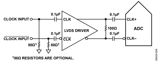
Figure 55. Differential LVDS Sample Clock
