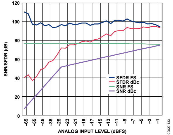
Figure 31. SNR/SFDR vs. Analog Input Level, f_{IN} = 97.3 MHz, 2.5 V p-p FS, AD9467-250
