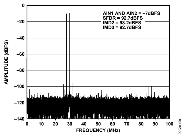
Figure 27. Two-Tone FFT with f_{IN1} = 170 MHz and f_{IN2} = 172 MHz, 2.5 V p-p FS, AD9467-200
