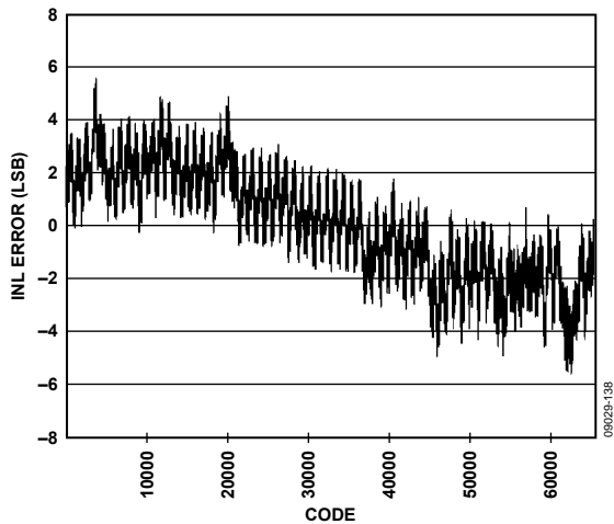
Figure 36. INL, f_{IN} = 4.3 MHz, 2.5 V p-p FS, AD9467-250
