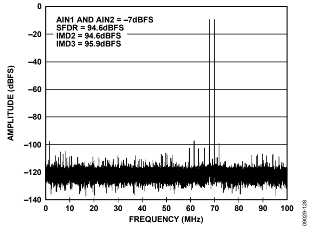
Figure 26. Two-Tone FFT with f_{IN1} = 70 MHz and f_{IN2} = 72 MHz, 2.5 V p-p FS, AD9467-200
