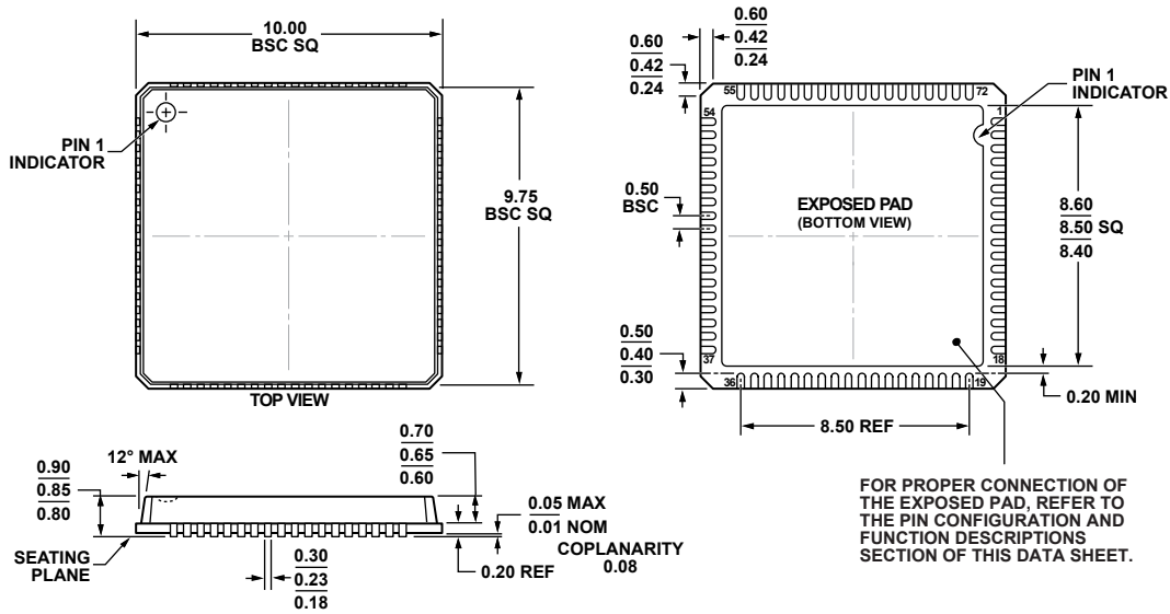
Figure 65. 72-Lead Lead Frame Chip Scale Package, Exposed Pad [LFCSP_VQ] 10 mm × 10 mm Body, Very Thin Quad (CP-72-5) Dimensions shown in millimeters
