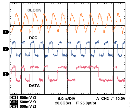
Figure 59. Output Timing Example in LVDS Mode (Default), AD9467-250
