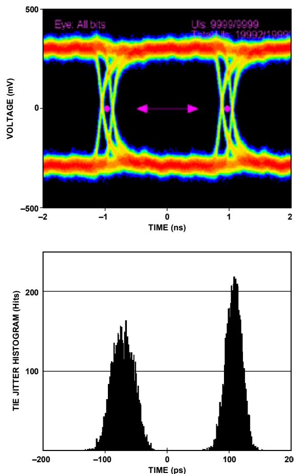
Figure 60. Data Eye for LVDS Outputs in ANSI-644 Mode with 6-Inch Trace Lengths on Standard FR-4, AD9467-250
