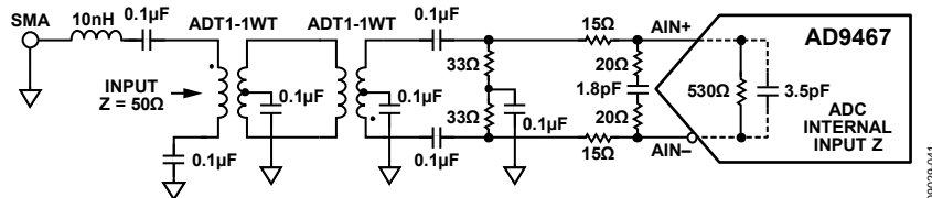
Figure 50. Differential Transformer-Coupled Configuration for IF Applications from 150 MHz to 300 MHz
