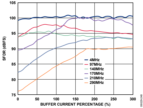
Figure 46. SFDR Performance vs. Buffer Current Percentage Over Analog Input Frequency, AD9467-250
