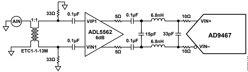
Figure 52. Differential Input Configuration Using the ADL5562
