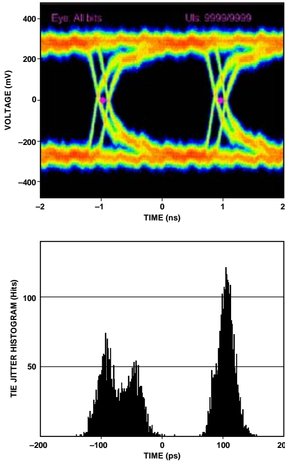
Figure 61. Data Eye for LVDS Outputs in ANSI-644 Mode with 18-Inch Trace Lengths on Standard FR-4, AD9467-250
