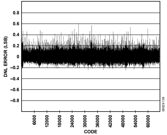
Figure 37. DNL, f_{IN} = 4.3 MHz, 2.5 V p-p FS, AD9467-250
