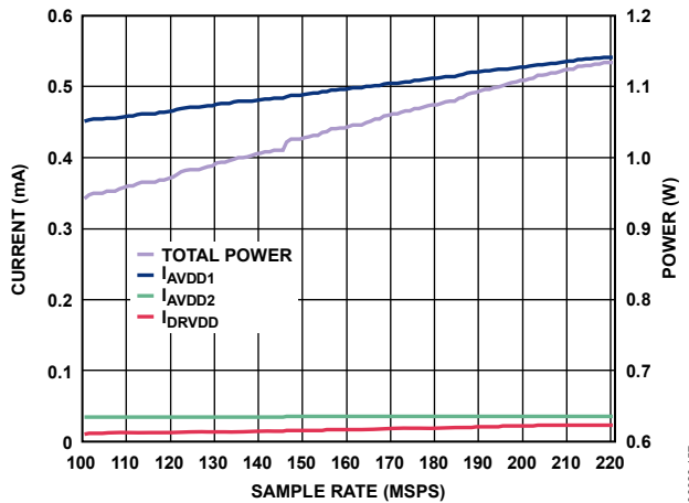
Figure 57. Supply Current vs. f_{SAMPLE} for f_{IN} = 5 MHz, AD9467-200
