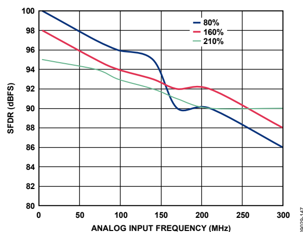
Figure 47. Buffer Current Sweeps, 2.5 V p-p, AD9467-250
