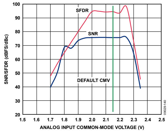
Figure 38. SNR/SFDR vs. Analog Input Common-Mode Voltage, A_{IN} = 100 MHz, 2.5 V p-p FS, AD9467-250
