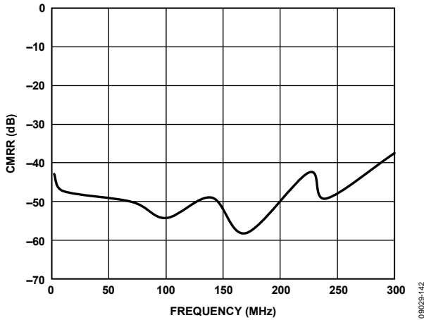
Figure 40. Common-Mode Rejection Ratio (CMRR), AD9467-250
