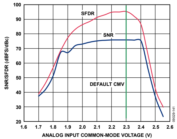
Figure 39. SNR/SFDR vs. Analog Input Common-Mode Voltage, A_{IN} = 100 MHz, 2.5 V p-p FS, AD9467-200
