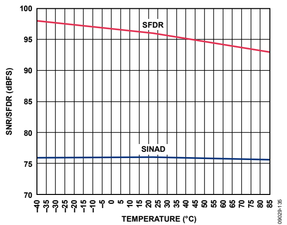
Figure 33. SINAD/SFDR vs. Temperature, f_{IN} = 97.3 MHz, 2.5 V p-p FS, AD9467-250
