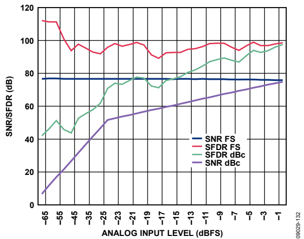
Figure 30. SNR/SFDR vs. Analog Input Level, f_{IN} = 97.3 MHz, 2.5 V p-p FS, AD9467-200
