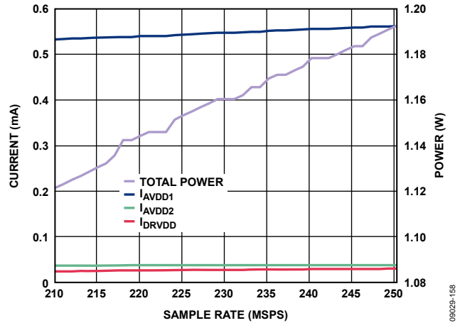
Figure 58. Supply Current vs. f_{SAMPLE} for f_{IN} = 5 MHz, AD9467-250
