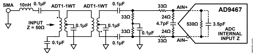
Figure 49. Differential Transformer-Coupled Configuration for Baseband Applications up to 150 MHz
