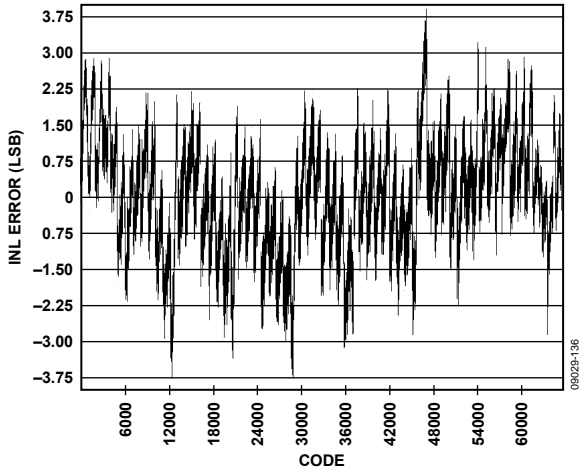
Figure 34. INL, f_{IN} = 4.3 MHz, 2.5 V p-p FS, AD9467-200
