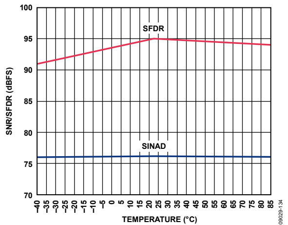
Figure 32. SINAD/SFDR vs. Temperature, f_{IN} = 97.3 MHz, 2.5 V p-p FS, AD9467-200
