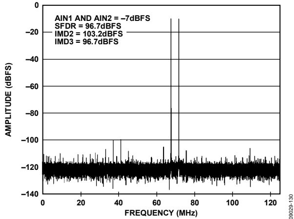
Figure 28. Two-Tone FFT with f_{IN1} = 70 MHz and f_{IN2} = 72 MHz, 2.5 V p-p FS, AD9467-250
