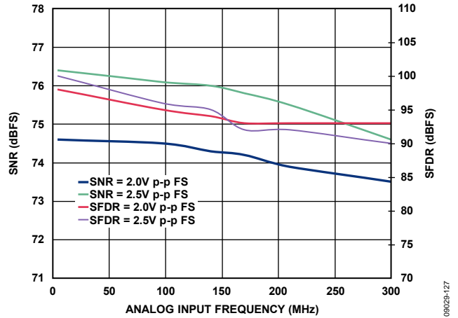
Figure 25. SNR/SFDR vs. f_{IN} , 2.0/2.5 V p-p FS, AD9467-250
