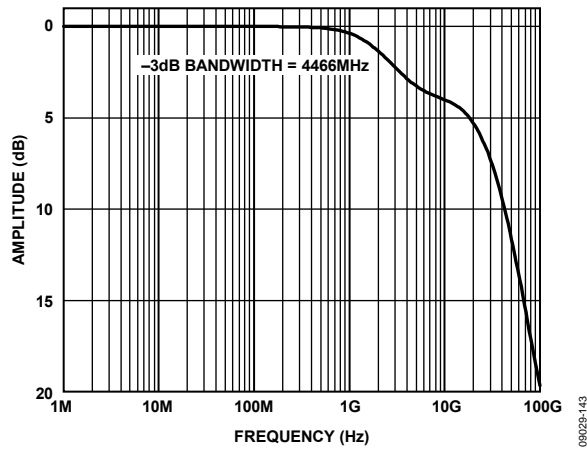
Figure 41. Analog Input Bandwidth AD9467-250
