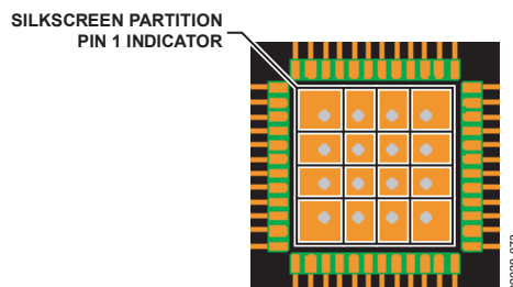
Figure 64. Typical PCB Layout
