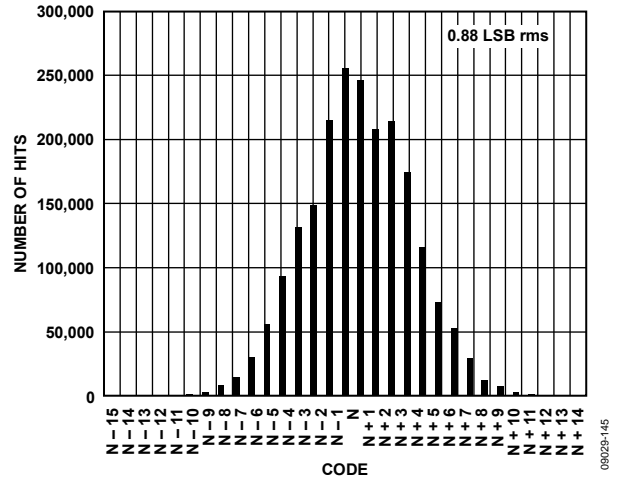
Figure 43. Input-Referred Noise Histogram, 2.5 V p-p FS, AD9467-200
