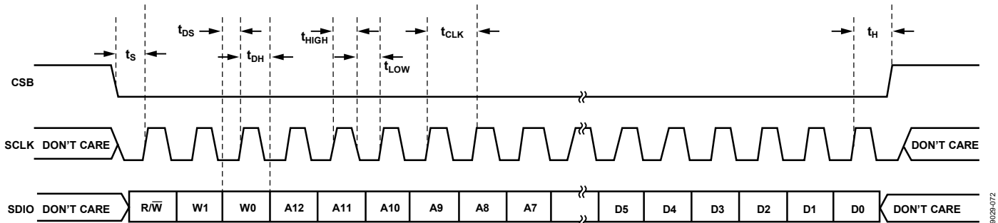
Figure 63. Serial Timing Details
